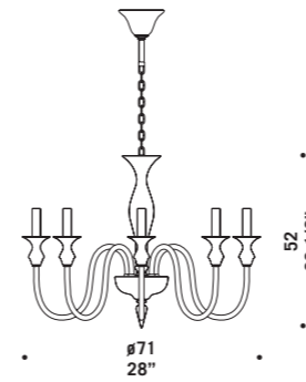
2599 K8 8 x max 46W E14 HSGSB/C/UB alogeno chiara clear halogen 8 x E14 LED LED light bulb
