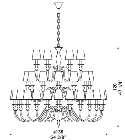
2599 K24+12+6 SHADE 42 x max 46W E14 HSGSB/C/UB alogena chiara clear halogen 42 x E14 LED LED light bulb
