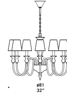
2599 K12 SHADE 12 x max 46W E14 HSGSB/C/UB alogena chiara clear halogen 12 x E14 LED LED light bulb
