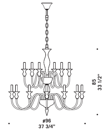
2599 K12+6 18 x max 46W E14 HSGSB/C/UB alogeno chiara clear halogen 18 x E14 LED LED light bulb
