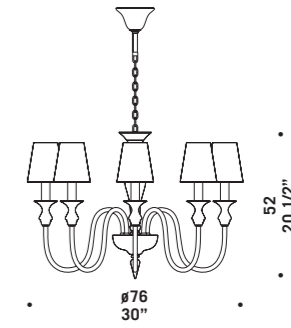
2599 K8 SHADE 8 x max 46W E14 HSGSB/C/UB alogena chiara clear halogen 8 x E14 LED LED light bulb
