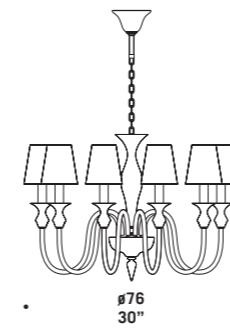
2599 K10 SHADE 10 x max 46W E14 HSGSB/C/UB alogena chiara clear halogen 10 x E14 LED LED light bulb
