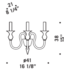
2599 A3 3 x max 46W E14 HSGSB/C/UB alogeno chiara clear halogen 3 x E14 LED LED light bulb
