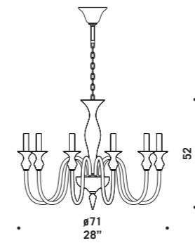
2599 K10 10 x max 46W E14 HSGSB/C/UB alogeno chiara clear halogen 10 x E14 LED LED light bulb
