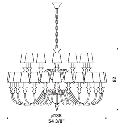
2599 K24+12 SHADE 36 x max 46W E14 HSGSB/C/UB alogena chiara clear halogen 36 x E14 LED LED light bulb
